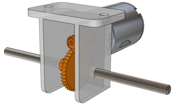
Drive mechanism
